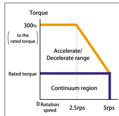
■ When operating D170-40-F/L at AC100V.
