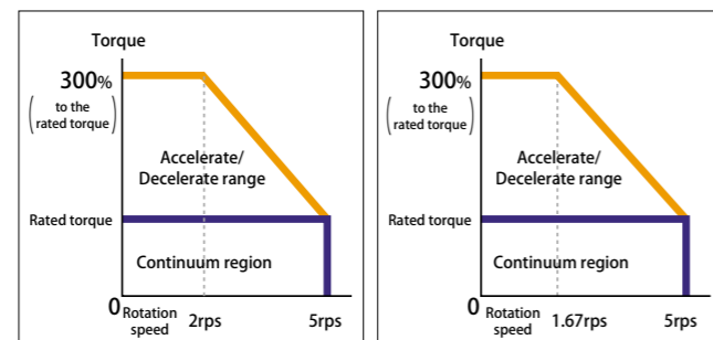
【ND】 When operating ND110-50-F/ND180-55-F at AC100V
