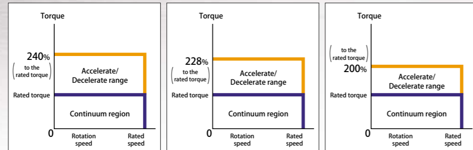
【ND-c】ND400-120-LC (1rps specification)
