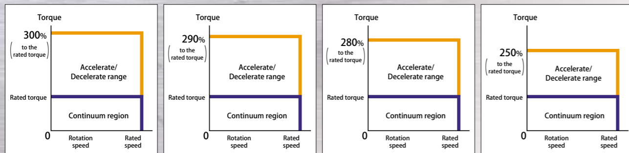
【ND-c】ND110-65-FC/ND110-85-FC ND140-70-LC/ND140-95-LC ND180-70-LC/ND180-95-LC ND250-70-LC
